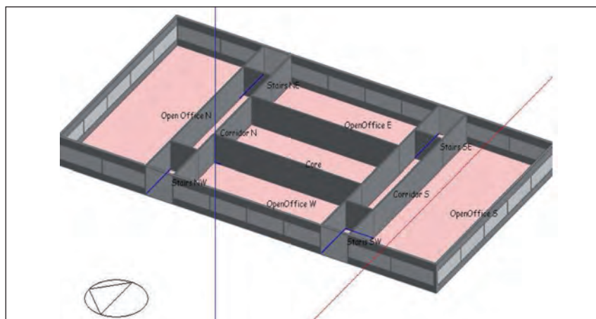
Figura 1. Screenshot del software DIALux ( www.dial.de ).
